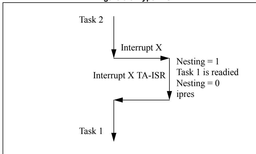
Figure 5-8 Type 2 ISR
