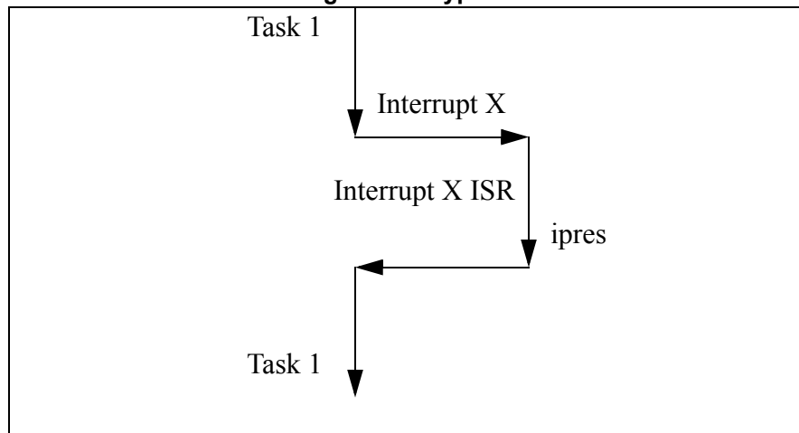
Figure 5-7 Type 1 ISR
